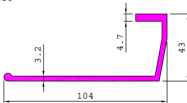
18558 1.438 kg/m
